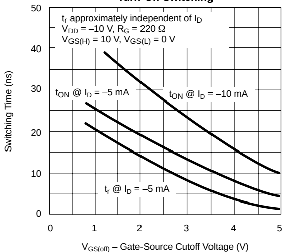
Turn-On Switching
