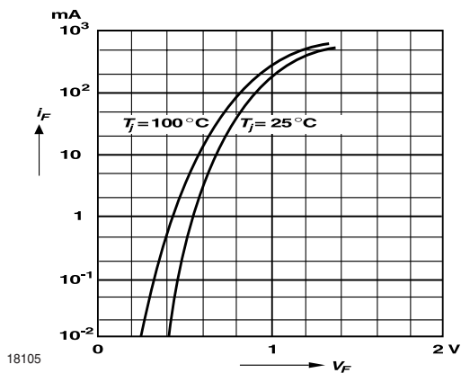
Fig. 1 Forward characteristics
