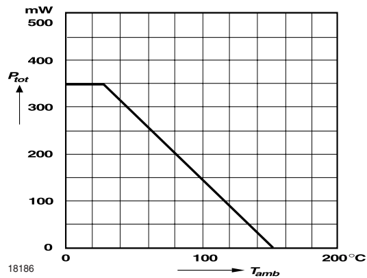
Fig. 3 Admissible Power Dissipation vs. Ambient Temperature
