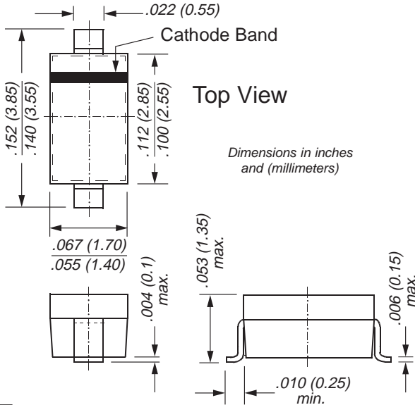
SOD-123
