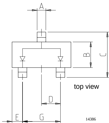
BAT54A, common anode
