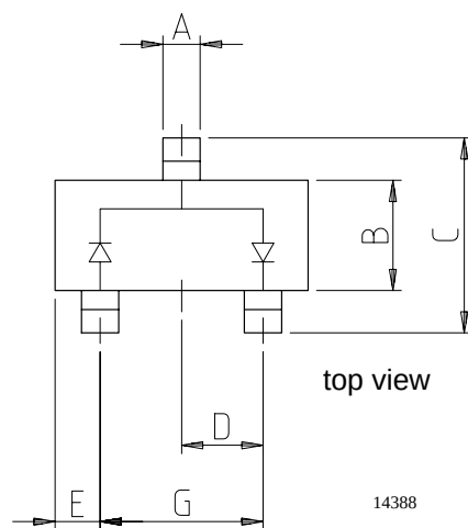
BAT54S, connected in series
