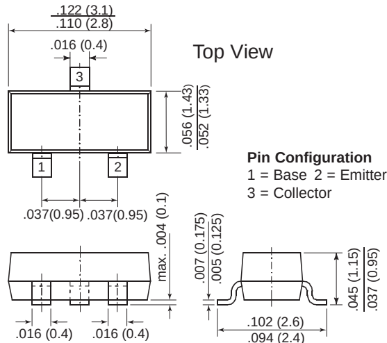
TO-236AB (SOT-23)
