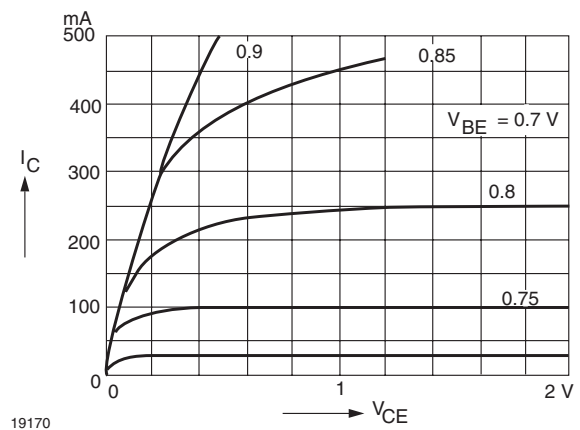
Figure 10. Common Emitter Collector Characteristics
