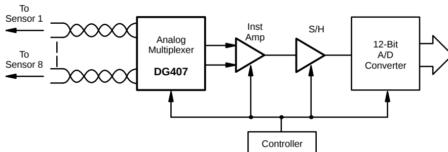
FIGURE 6. Measuring low-level analog signals is more accurate when using a differential multiplexing technique.
