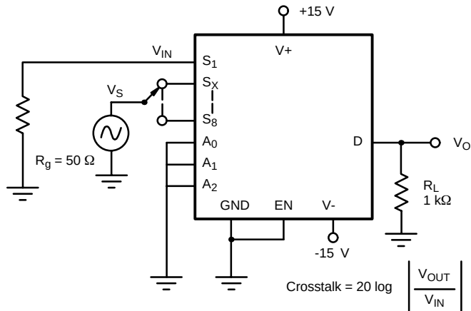
FIGURE 7. Crosstalk
