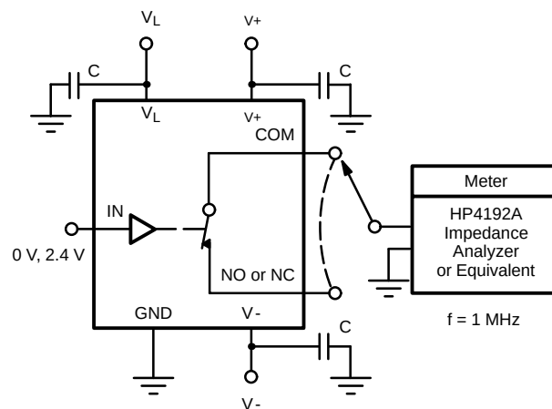
Figure 8. Source/Drain Capacitances
