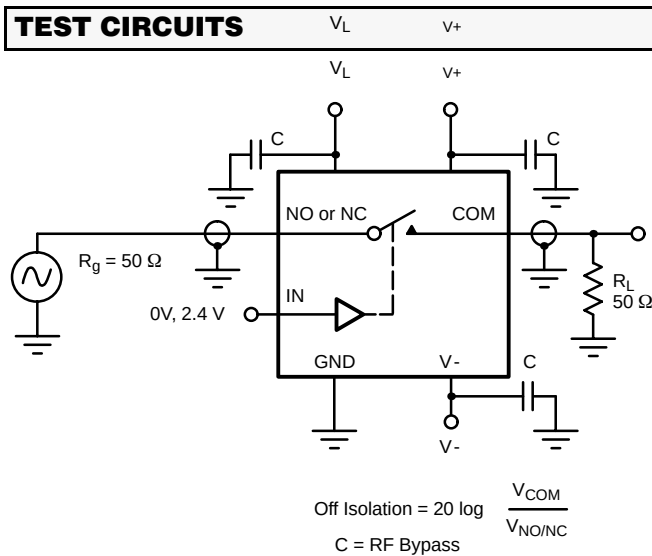
Figure 7. Off Isolation
