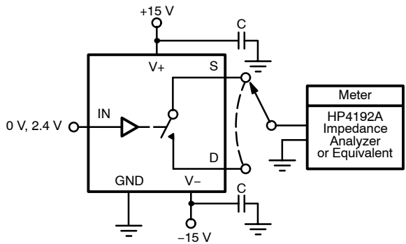
FIGURE 6. Source/Drain Capacitances
