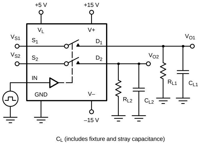
FIGURE 1. Switching Time
