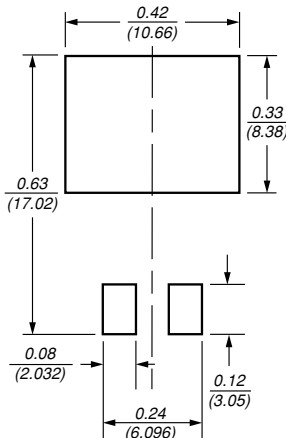
Mounting Pad Layout
