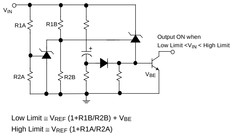
Fig. 23 – Over-Voltage / Under-Voltage Protection Circuit
