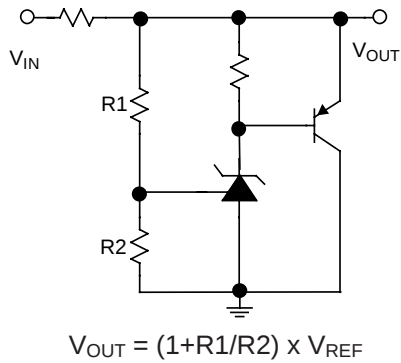
Fig. 21 – High-Current Shunt Regulator
