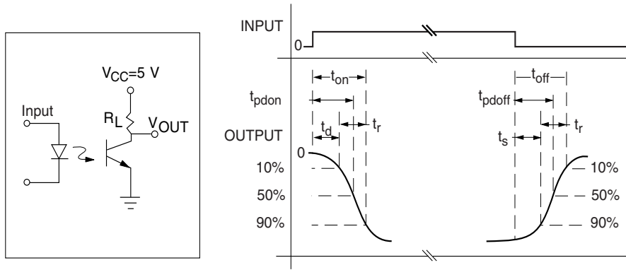
Fig. 11 Switching Time Test Schematic and Waveform
