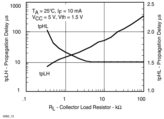
Fig. 13 Propagation Delay vs. Collector Load Resistor
