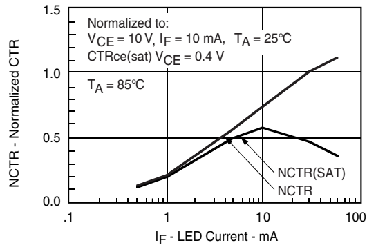
Fig. 6 Normalized Non-saturated and saturated CTR vs. LED Current
