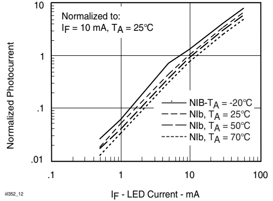
Fig. 12 Normalized Photocurrent vs. I_F and Temp.
