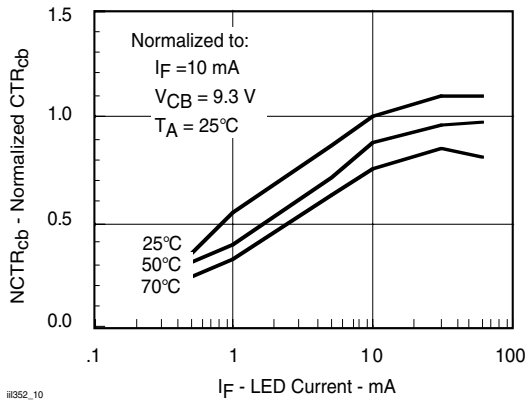
Fig. 10 Normalized CTR_{cb} vs. LED Current and Temperature
