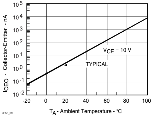
Fig. 9 Collector-Emitter Leakage Current vs.Temp.
