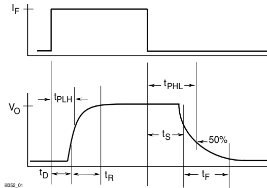
Fig. 1 Switching Waveform
