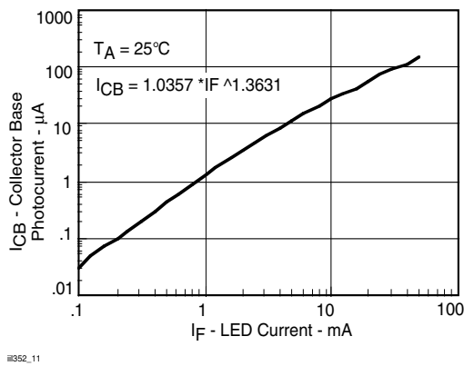
Fig. 11 Collector-Base Photocurrent vs. LED Current
