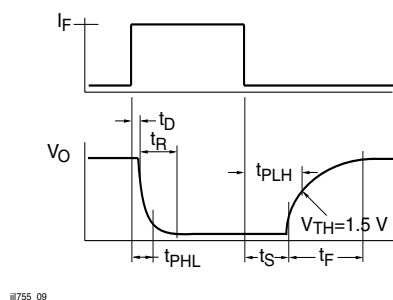
Figure 9. Switching Waveform
