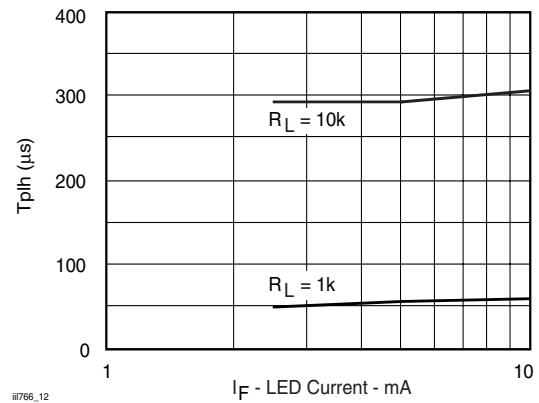
Figure 12. t_{plh} vs. Forward Current
