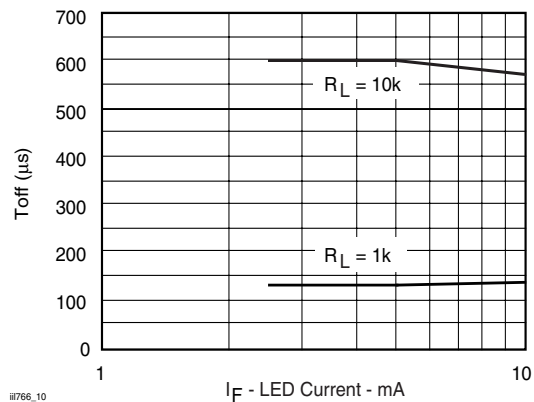
Figure 10. t_{off} vs. Forward Current
