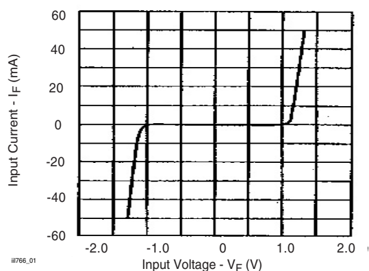
Figure 1. Input Characteristics
