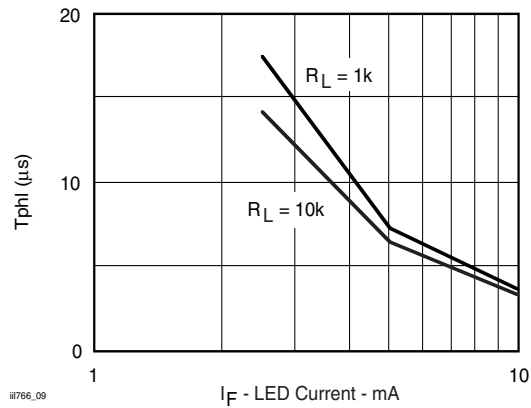
Figure 9. t_{on} vs. Forward Current
