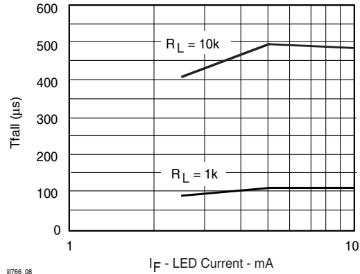
Figure 8. t_{fall} vs. Forward Current
