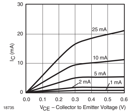
Figure 5. Normalized Current vs. Collector Emitter Saturation Voltage
