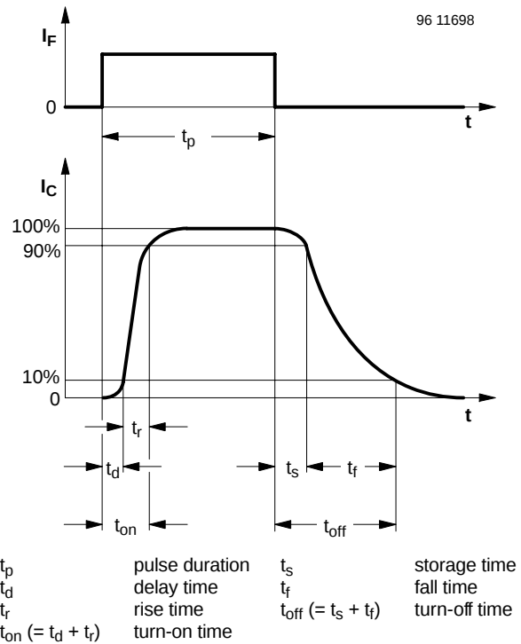
Figure 3. Switching times
