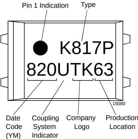
Figure 14. Marking example
