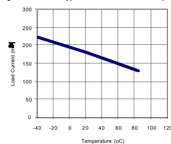
Figure 4. Form B_Typical Load Current vs. Temperature
