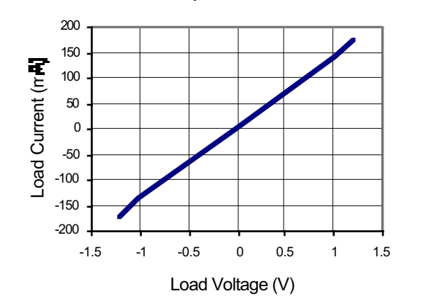
Figure 2. Form A_Typical Load Current vs. Load Voltage (Ambient Temp.= 25°C; IF=5 mA)
