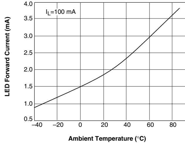
Figure 1. LED Forward Current for Switch Turn-on/off
