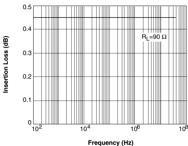
Figure 6. Insertion Loss (per Pole) vs. Frequency
