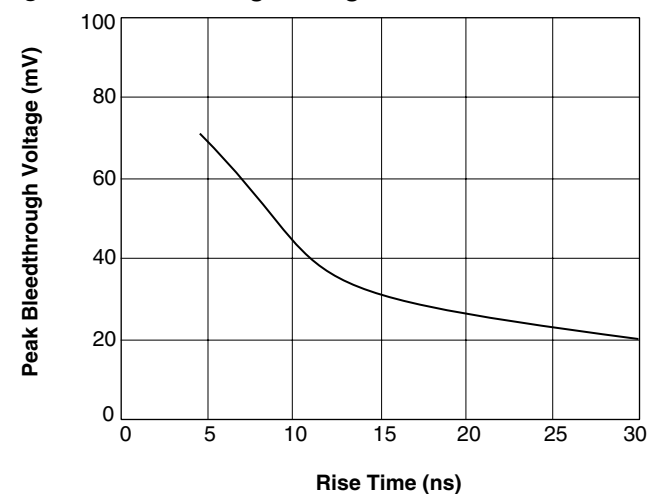
Figure 8. Bleed-through Voltage vs. Rise Time
