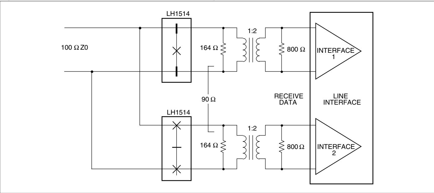
Figure 15. T1 Multiplexer Receive Data (Interface 1, Operating) Features
