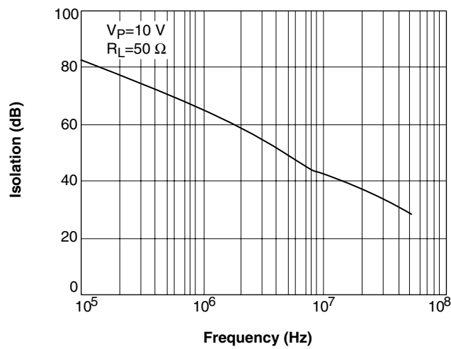
Figure 5. Output Isolation
