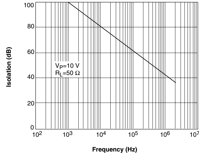
Figure 9. Output Isolation
