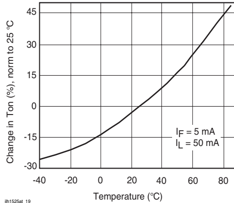
Figure 20. Turn-on Time vs. Temperature
