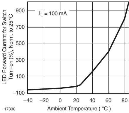
Figure 5. LED Current for Switch Turn-on vs. Temperature
