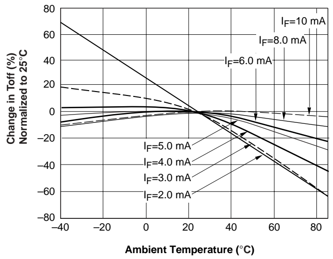
Figure 9. Turn-off Time vs. Temperature
