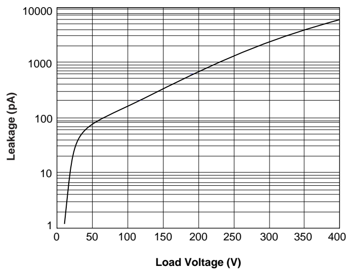
Figure 8. Leakage Current vs. Applied Voltage
