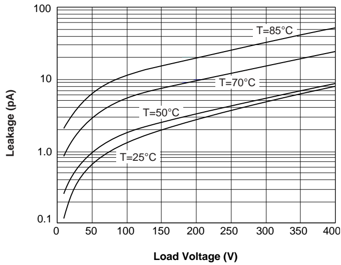
Figure 7. Leakage Current vs. Applied Voltage
