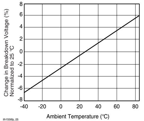
Figure 5. Switch Breakdown Voltage vs. Temperature
