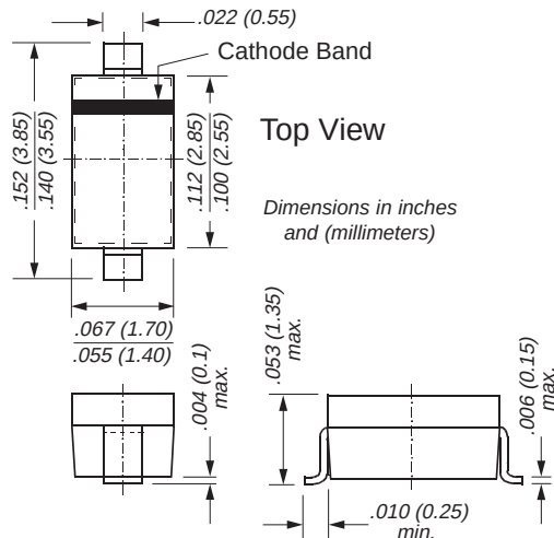
SOD-123
