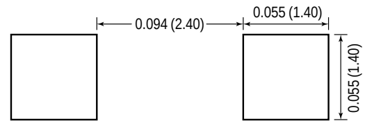
Mounting Pad Layout
