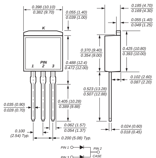
TO-262AA (MBRB10H150CT-1)
