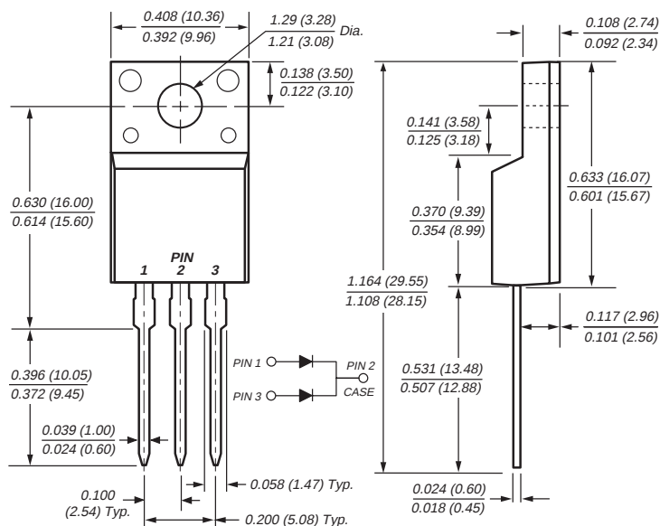
ITO-220AB (MBRF10H150CT)
