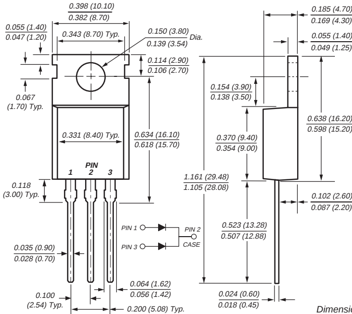
ITO-220AB (MBRF10H150CT)
