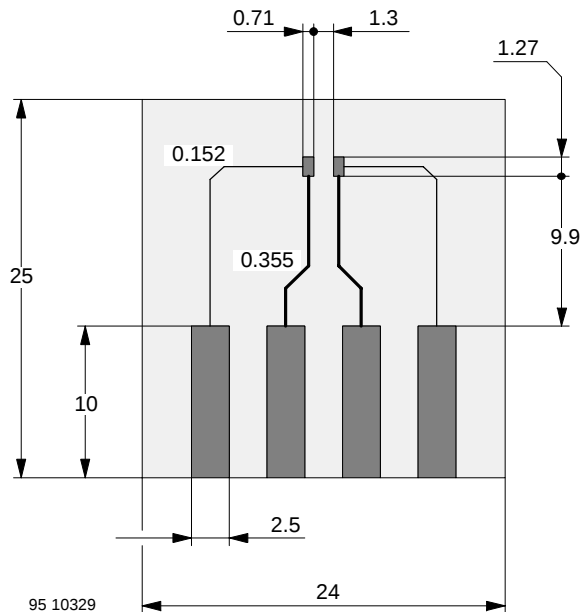
Figure 1. Board for R thJA definition (in mm)
