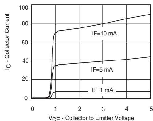
Figure 2. Typical I_C vs. V_{CE}
