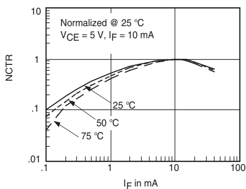
Figure 4. Typical NCTR vs. LED Current
