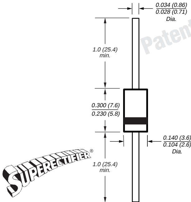
DO-204AC (DO-15)
