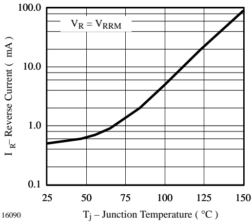
Figure 1. Max. Reverse Current vs. Junction Temperature
