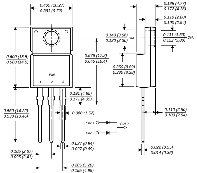
ITO-220AB (SBLF16xxCT)
