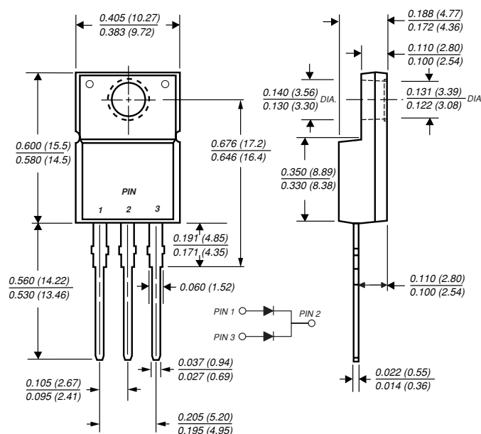
ITO-220AB (SBLF25LxxCT)
