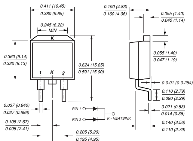
TO-263AB (SBLB25LxxCT)
