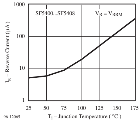
Figure 8. Max. Reverse Current vs. Junction Temperature
