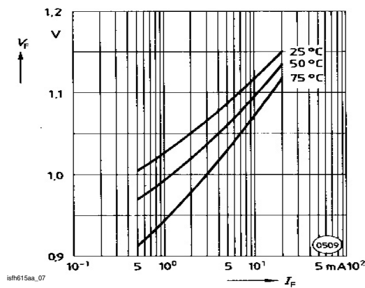
Figure 7. Diode Forward Voltage (typ.) vs. Forward Current
