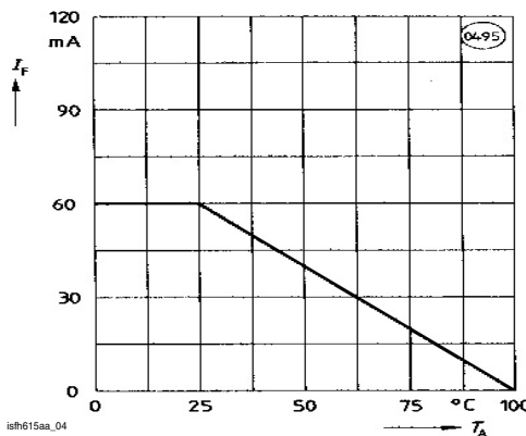
Figure 4. Permissible Diode Forward Current vs. Ambient Temperature
