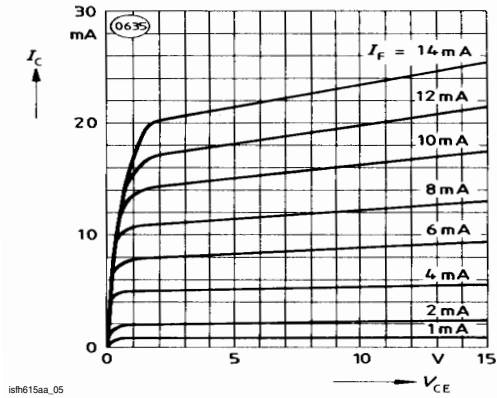
Figure 5. Output Characteristics (typ.) Collector Current vs. Collector-Emitter Voltage
