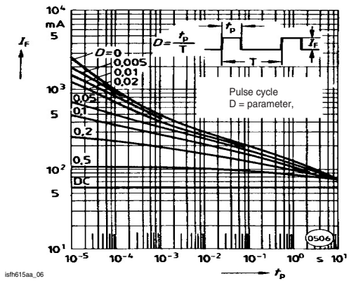
Figure 6. Permissible Pulse Handling Capability Forward Current vs. Pulse Width
