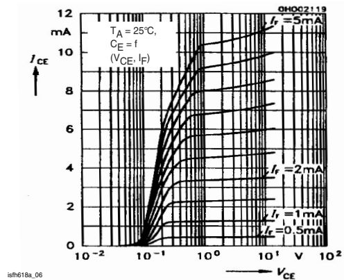
Figure 9. Output Characteristics
