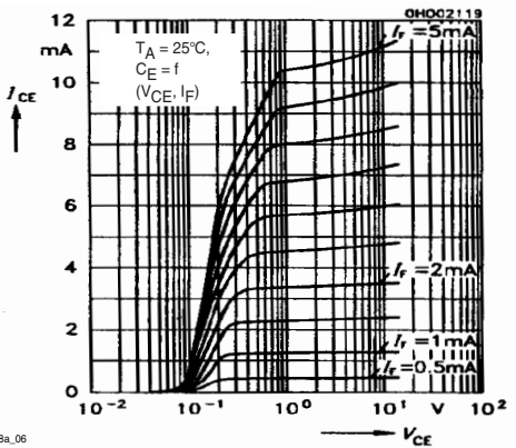
Fig. 9 Output Characteristics
