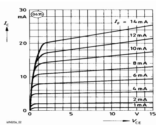
Fig. 3 Output Characteristics (typ.) Collector Current vs. Collector-Emitter Voltage
