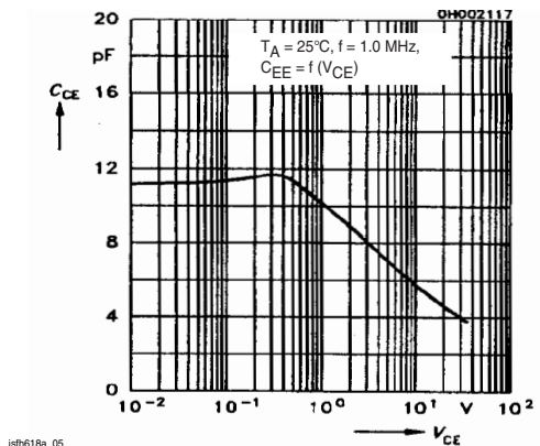
Figure 7. Transistor Capacitance
