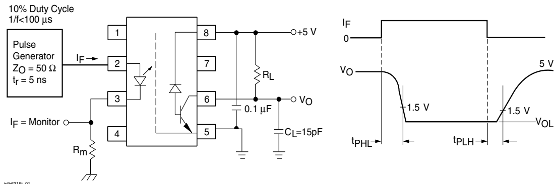
Fig. 1 Test Circuit for Switching Times
