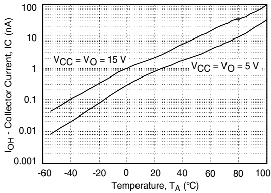
Fig. 9 Logic high output current vs. temperature
