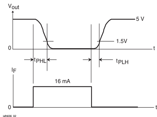
Figure 2. Switching Time Measurement
