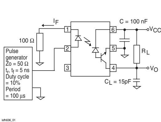
Figure 1. Test Set-up
