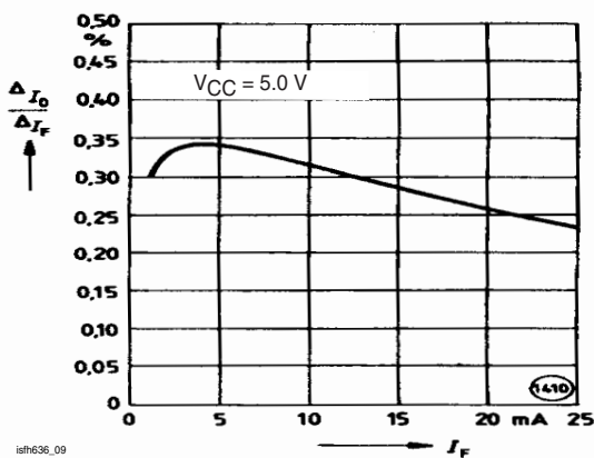
Fig. 9 Small Signal Transfer Ratio vs. Forward Current
