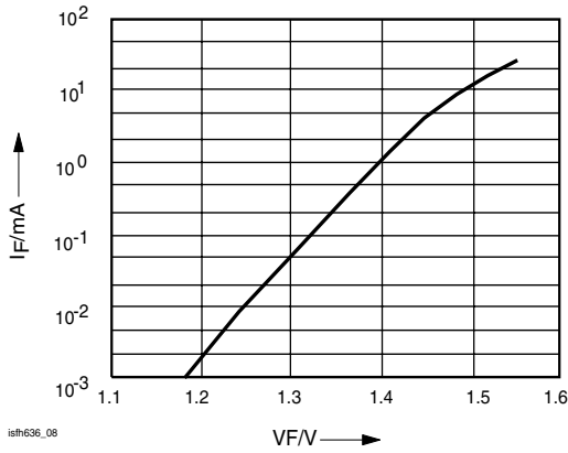
Fig. 8 Forward Current of Emitting Diode vs. Forward Voltage
