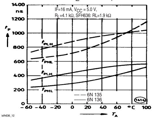
Fig. 12 Delay Times vs. Ambient Temperature
