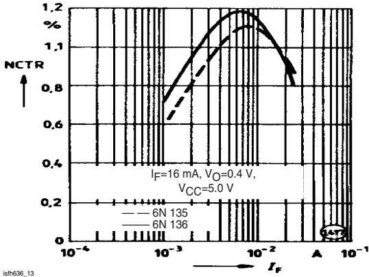
Fig. 13 Current Transfer Ratio (normalized) vs. Forward Current
