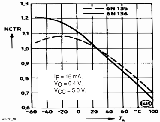
Fig. 10 Current Transfer Ratio (normalized) vs. Ambient Temperature
