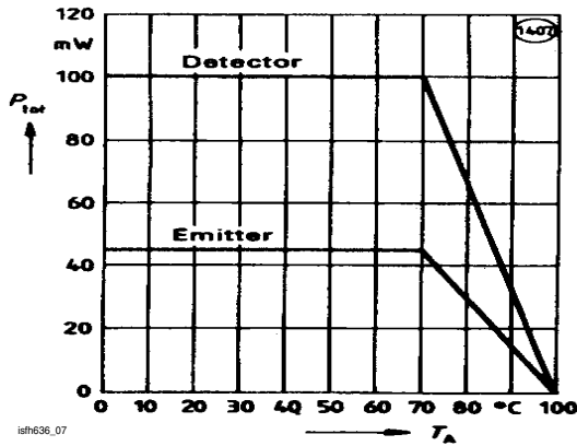
Fig. 7 Permissible Total Power Dissipation vs. Ambient Temperature
