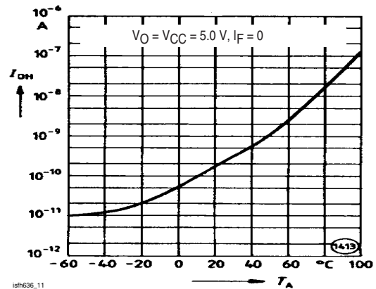
Fig. 11 Output Current (high) Vs. Ambient Temperature
