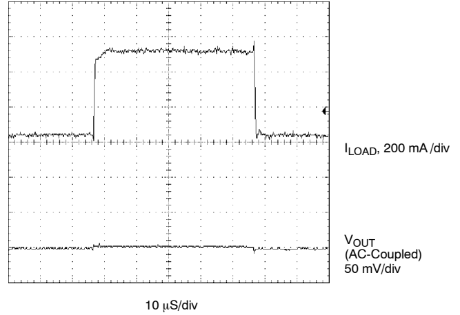
Load Transient, PWM Mode, I_{LOAD} = 30 to 500\text{ mA} , L = 2.2\text{ μH} , MODE = HIGH
