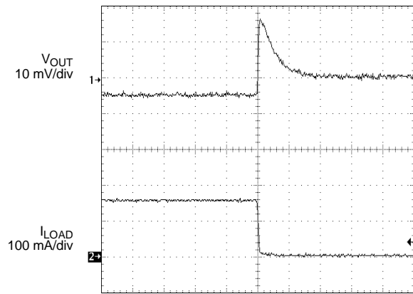
Load Transient Response-2
