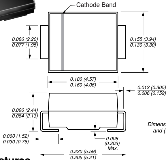
DO-214AA (SMB)
