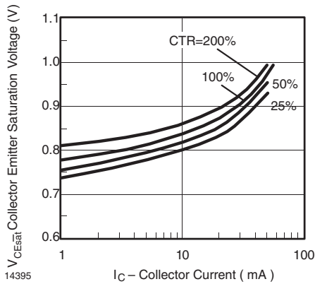
Fig. 11 Collector-Emitter Saturation Voltage vs. Collector Current
