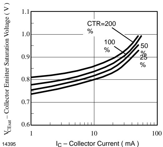
Figure 11. Collector-Emitter Saturation Voltage vs. Collector Current
