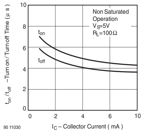
Fig. 15 Turn on / off Time vs. Collector Current
