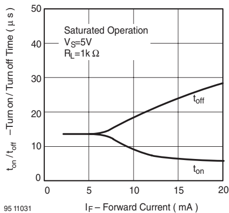
Fig. 14 Turn on / off Time vs. Forward Current
