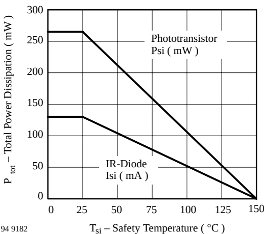
Figure 1. Derating diagram
